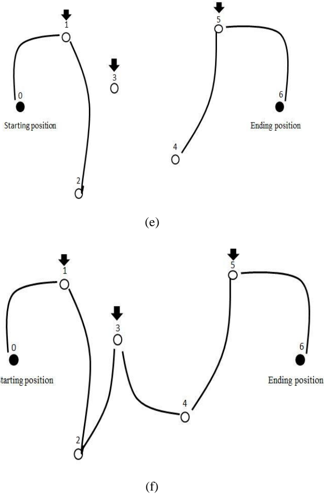
Fig.2. Shortest Path Algorithm (a) Grid Layout (b) Move to the nearest item from the starting position (c) Move to the nearest item from the ending position (d) Move to the next item through the shortest path (e) Move to the next item through the shortest path (f) Shortest path.
