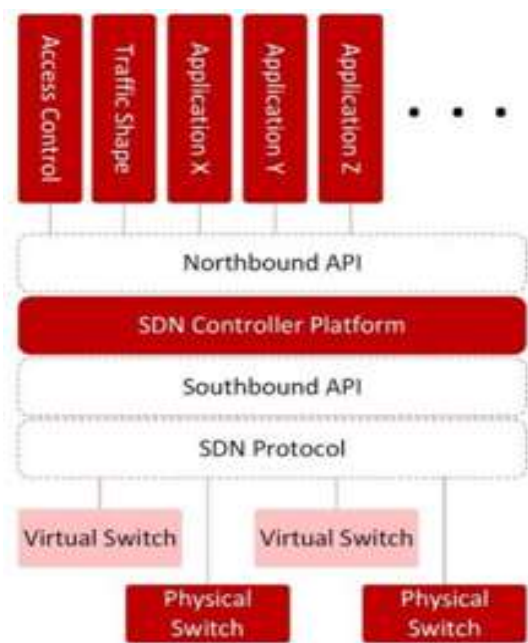
FIGURE 1. NORTHBOUND AND SOUTHBOUND INTERFACES IN AN SDN ARCHITECTURE.
